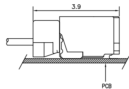
MATED CONDITION
